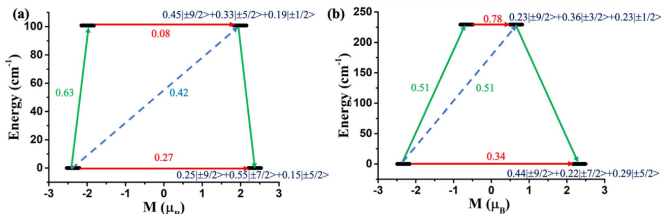
Fig. 7 The mechanism of magnetization relaxation of (a) [U(Tp^{Me_2})_2(THF)_2] (7) and (b) [U(Tp^{Me_2})_2CH_2Ph] (9). The red arrows denote the QTM via the ground state and TA-QTM via the first excited state. The sky-dotted arrow represents the Orbach process. The green arrows indicate the most possible pathway of magnetisation relaxation.
