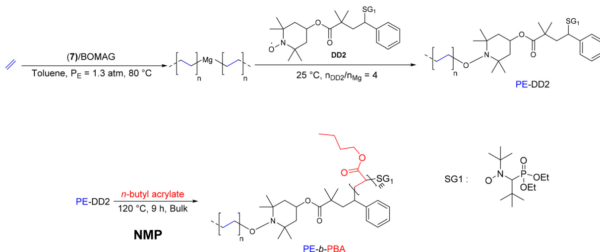
Scheme 13 Synthesis of \text{PE-}b\text{-PBA} block copolymers by combining CTP and NMP. 35
