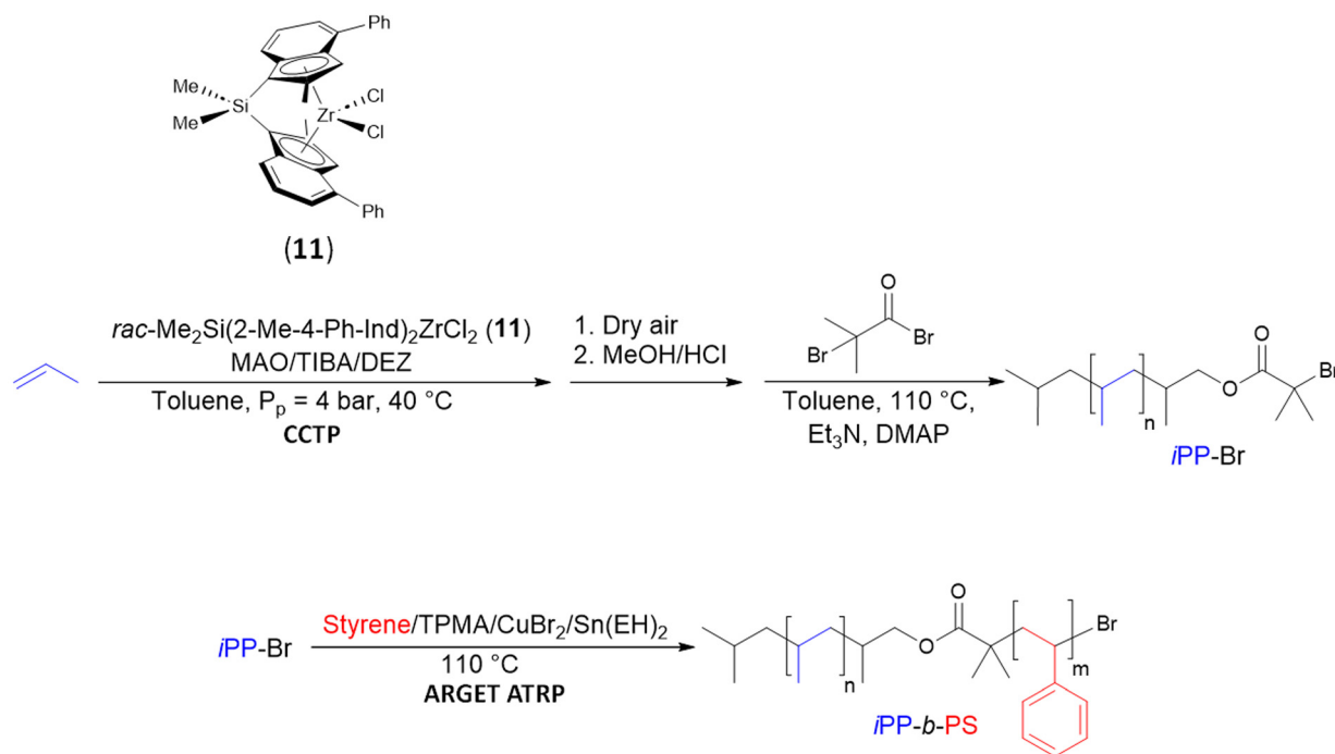
Scheme 12 Synthesis of i\text{PP-}b\text{-PS} block copolymers by combining CTP and ARGET ATRP. 34
