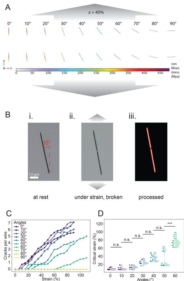
Fig. 2 (A) FEA results of wires with different orientations when subjected to 40% strain. The colors in the wires represent the experienced von Mises stress. (B) Process flow used for the mechanical characterization of wires subjected to strain. (i) Example of a pristine wire at rest, (ii) wire experiencing strain and breaking as a result thereof, (iii) the processed image reveals the detection of 2 distinct segments, confirming the cracking of the wire. (C) Average number of cracks per wire for each angle group, as a function of strain. Data points were taken every 5% strain. N = 5 to 18, depending on how many wires would fit in the field of view for a given angle and strain. (D) The critical strain at which each microwire first breaks, across all orientations. Each scattered dot represents a single wire breaking, and the violin plot shows the distribution. Since photographs were taken every 5% only, the dots are placed in the middle of the interval between the last strain without breakage and the interval at which breakage was noted, with an artificial jitter for visualization. Angles from 70° to 90° are not presented as no cracks were seen. Statistical significance was determined using Kruskal–Wallis test with Dunn's post hoc test (** p < 0.001 ).
