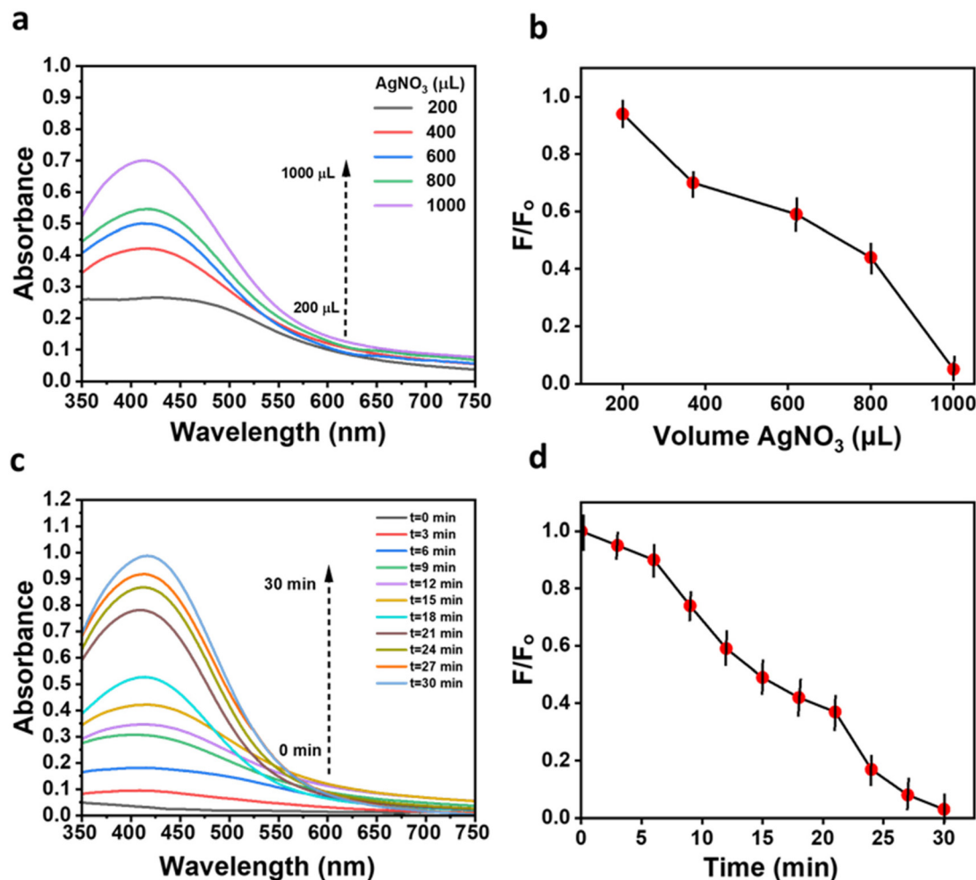
Fig. 4 (a) Extinction spectrum and (b) the relative fluorescence intensity of the CD@AgNP hybrid sample as a function of different volumes of AgNO 3 (200 400, 600 800, and 1000 μL). (c) Time evolution of the UV-visible spectrum and (d) the relative fluorescence intensity of the CD@AgNP hybrid. 1000 μL of AgNO 3 (20 mM) and the Ag + : CD volume ratio of 1:4 were used for the synthesis. Standard deviations are for three replicates. \lambda_{\text{ex}} = 350 nm and \lambda_{\text{em}} = 409 nm were used in fluorescence studies.
