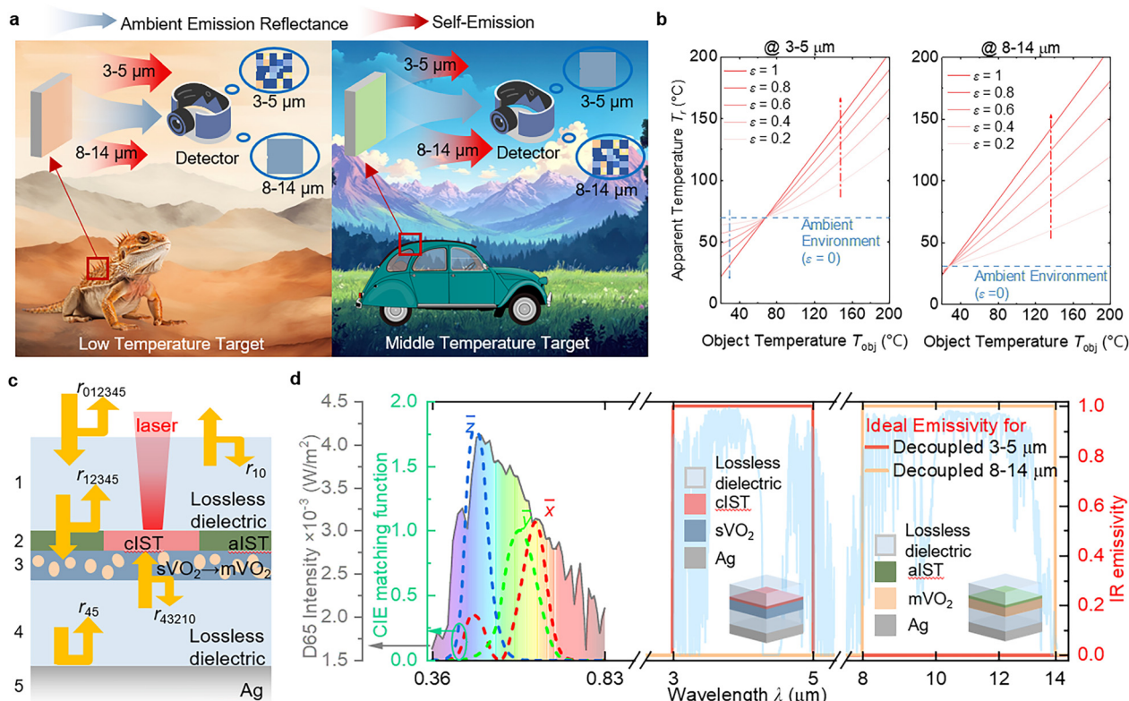
Fig. 1 Schematic of the decoupled camouflage principle and ideal spectral characteristics. (a) Potential applications of multi-band decoupled thermal camouflage for low-temperature and mid-temperature targets. The blue arrow represents the reflection of thermal radiation projected to the surface of the thermal camouflage device by the ambient environment, including the thermal radiation of the surrounding environment and solar radiation, and the red arrow represents the thermal self-emission of the thermal camouflage device. (b) Apparent temperature, T_r , as a function of emissivity, \epsilon , and the object temperature, T_{obj} , in the range of 3–5 μm and 8–14 μm. Here, we assume the device is a gray body, and the blue dash line is the apparent temperature of the ambient environment radiation when the target's emissivity is 0 according to eqn (1), and the red and blue dash dot lines are the emissivity modulation trends with increasing average emissivity for the corresponding spectral region. (c) Schematic of the heterogeneous phase-change material integrated thermal emitter. The green region and red region indicate the local phase-change process of IST via laser stimulation. The blue region and light orange region represent the uniform phase transition of VO 2 from sVO 2 to mVO 2 upon heating, and r_{ij} denotes the reflectance coefficient from the i th layer into the j th layer and the numbers on the left indicate the serial number of each layer. (d) D65 light source power density and the ideal decoupled IR emissivity the range of 3–5 μm and 8–14 μm, where the dash lines are CIE matching functions. The light blue lines represent atmospheric transmittance, indicating that 3–5 and 8–14 μm are the commonly used atmospheric windows for infrared detection with high infrared transmittance.
