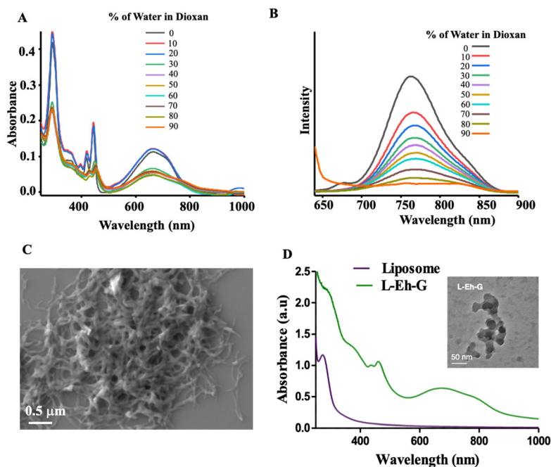
Fig. 1 A. Absorption spectra of Eh-G at different vol% of water in dioxane. B. Emission spectra of Eh-G at different vol% of water in dioxane ( \lambda_{\text{exc}} = 620 \text{ nm} ). C. FE-SEM image of Eh-G in 90 vol% water in dioxane. D. Absorption spectra of plain liposomes and liposomes encapsulated with Eh-G ( L-Eh-G ). The TEM image of L-Eh-G is shown in the inset of D.
