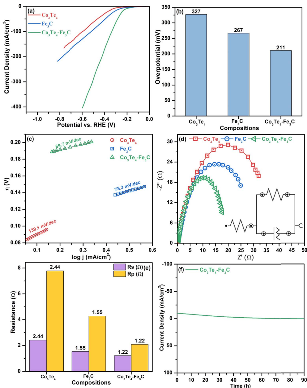
Fig. 5 HER electrocatalysis: (a) LSV curves, (b) bar chart of overpotential at 10 mA cm -2 current density, (c) Tafel plots, (d) EIS plots, (e) comparison of R_p and R_s , and (f) stability ( i-t ) curve of \text{Co}_3\text{Te}_4 , \text{Fe}_3\text{C} , and \text{Co}_3\text{Te}_4\text{-Fe}_3\text{C} .
