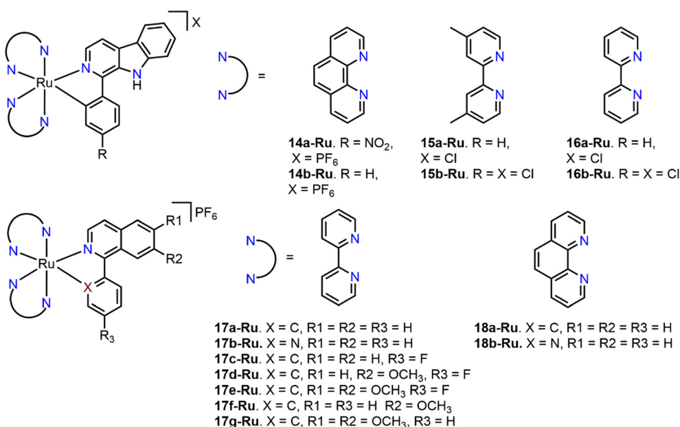
Fig. 10 Ru(II) \text{C}^{\wedge}\text{N} compounds with cyclometalated ligands derived from \beta -carboline ( 14a-Ru–16b-Ru ) and isoquinolines ( 16a-Ru–18b-Ru ).
