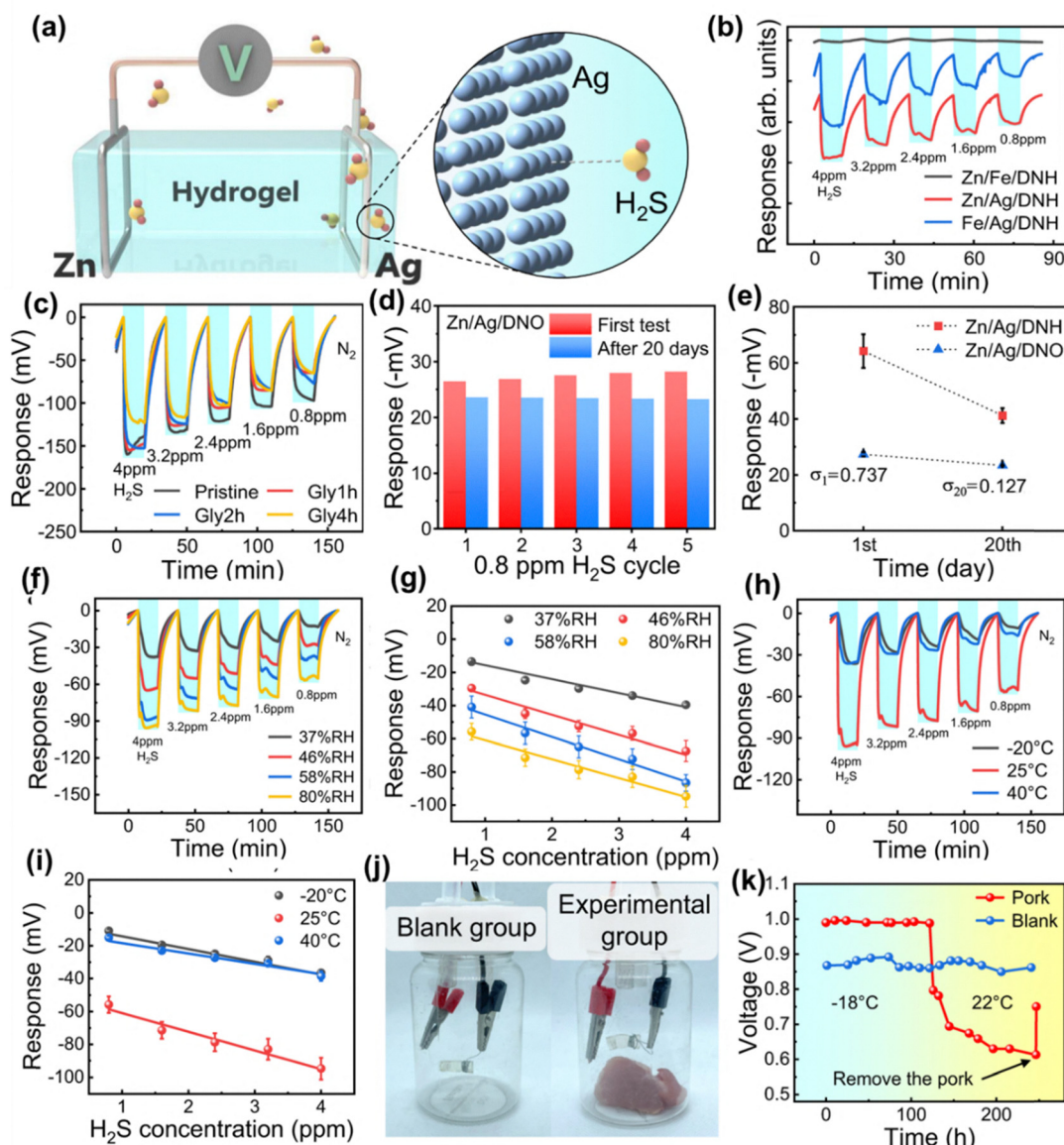
Fig. 13 (a) Schematic illustration of the self-powered \text{H}_2\text{S} sensor based on Zn/Ag electrodes and a hydrogel electrolyte. (b) Comparison of \text{H}_2\text{S} sensing responses for different electrode configurations (Zn/Ag, Zn/Fe, and Fe/Ag). (c) Dynamic response of the sensor to various \text{H}_2\text{S} concentrations (0.8–4 ppm) with different hydrogel modifications. (d) Long-term stability test showing sensor response over 20 days with repeated \text{H}_2\text{S} exposure cycles. (e) Signal degradation analysis of Zn/Ag and Zn/Fe electrodes over time under continuous \text{H}_2\text{S} exposure. (f) Humidity-dependent response of the sensor across different relative humidity (RH) levels. (g) Sensitivity comparison of the sensor under varying humidity conditions (37–80% RH). (h) Temperature-dependent \text{H}_2\text{S} sensing response at -20^\circ\text{C} , 25^\circ\text{C} , and 40^\circ\text{C} . (i) Effect of temperature variations on sensor response across different \text{H}_2\text{S} concentrations. (j) Application of the sensor in food spoilage detection, comparing a blank group with pork samples. (k) Real-time voltage response of the sensor during food spoilage monitoring, showing \text{H}_2\text{S} accumulation over time. Reproduced with permission, 60 Creative Commons Attribution 4.0 International License Copyright © 2023 Springer Nature.
