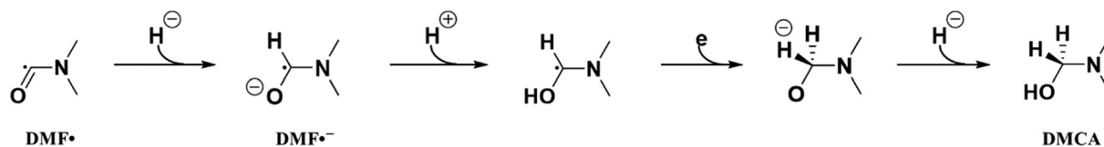
Fig. 5 Schematic of the DMCA preparation from \text{DMF}^\bullet generated by the DBD-catalyzed MOFs preparation in DBD liquid plasma. Reproduced from ref. 61 with permission from RSC, copyright 2019.
