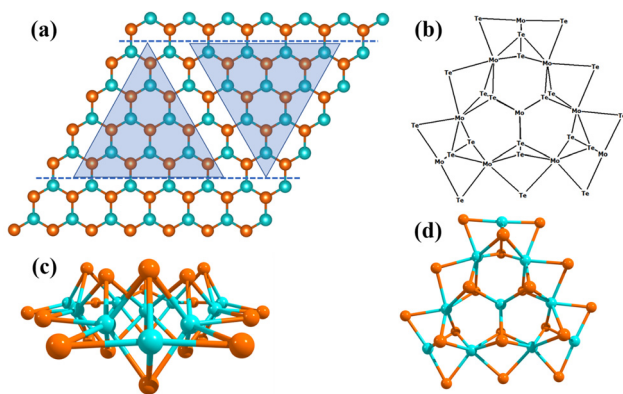
Fig. 1 (a) The equilibrium 2D monolayer MoTe 2 TMD with a Te–Mo–Te tri-layer structure. The two horizontal blue color dashed lines indicate terminations along the (10 \bar{1} 0) Mo-edge and (10 \bar{1} 0) Te-edge. The two triangles represent the terminations for Mo-edge and Te-edge clusters. It includes a non-periodic molecular cluster with an active Te-edge and a non-periodic molecular cluster with an active Mo-edge. (b) The molecular cluster model system of the 2D monolayer MoTe 2 TMD represented schematically. (c) A side view of the chosen Mo 10 Te 21 non-periodic triangular molecular cluster. (d) A top view of the MoTe 2 TMD Mo-edge cluster.
