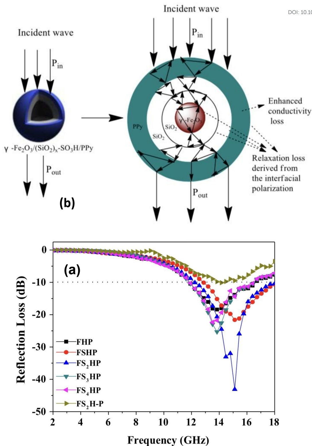
Figure 22 (a) Variation of R_L of \gamma\text{-Fe}_2\text{O}_3/(\text{SiO}_2)_x\text{-SO}_3\text{H} /polypyrrole (referred as \text{FS}_x\text{HP} , where x=0,1,2,3,4 ) core/shell/shell microspheres and \text{FS}_2\text{H-P} (physical blend of \text{FS}_2\text{H} and PPy) with the frequency ( d = 2\text{ mm} ), and (b) Physical model of the effects of core/shell/shell structures on the microwave absorption. 390 Reproduced with permission from Springer.
