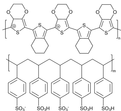
Fig. 10 (a) Chemical structures of PEDOT and PSS.
