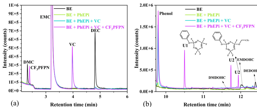
Fig. 6 (a) Gas chromatograms obtained from 10 s SPME sampling of extracted BE or electrolyte containing PhEPI, PhEPI + VC or PhEPI + VC + \text{CF}_3\text{PFPN} . (b) Gas chromatograms obtained from 600 s SPME sampling of extracted BE or electrolyte containing PhEPI, PhEPI + VC or PhEPI + VC + \text{CF}_3\text{PFPN} . The postulated structures of the compounds are represented in the figures at the retention time of the corresponding peaks.
