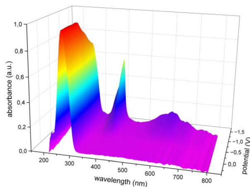
Fig. 2 Spectroelectrochemical measurements of MVCl_2 illustrating the appearance of MV^{+\cdot} in TFE.
