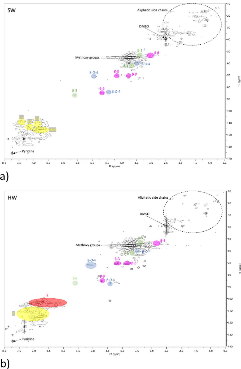
Fig. 1 HSQC spectrum of (a) softwood lignin (SW) and (b) hardwood lignin (HW).
