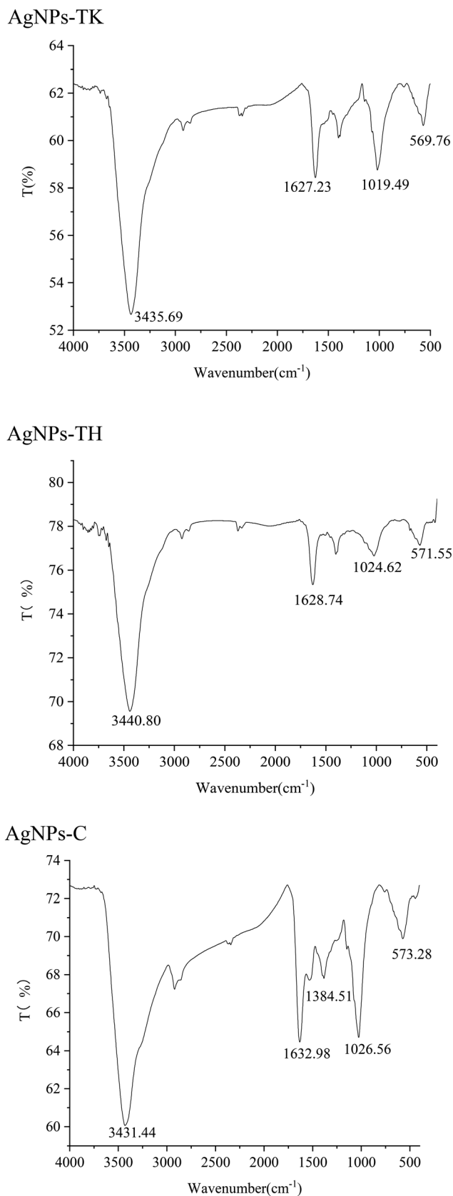
Fig. 7 Fourier-transform infrared absorption spectra of three kinds of AgNPs.
