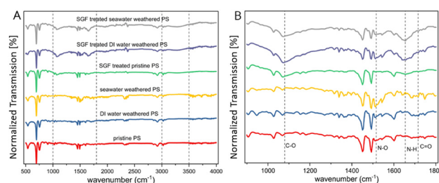
Fig. 1 ATR-FTIR spectrum of surface chemical functional groups on all particles. A. Spectrum of all types of particles at full wavenumber range from 500–4000 cm -1 and B. spectrum of wavenumber range from 900–1800 cm.
