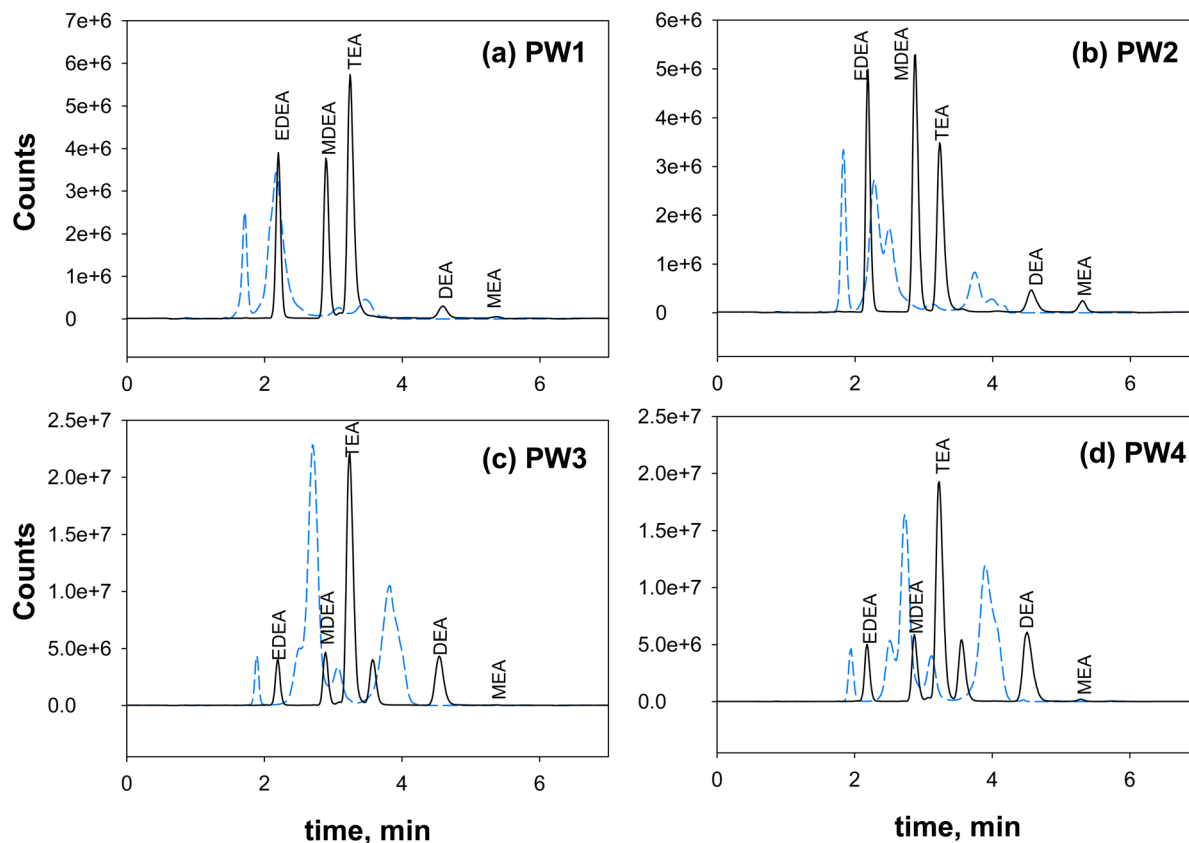
Fig. 2 Total ion chromatograms (TIC) of ethanolamines ( 15\ \mu\text{g L}^{-1} ) in PW-Mar samples ((a) PW1, (b) PW2, (c) PW3, (d) PW4) showing improved method sensitivity and peak resolution using the proposed SPE procedure. X-axis is time (min) and y-axis is counts/signal intensities. Peaks from left to right: EDEA, MDEA, TEA, DEA, MEA. Black line: chromatogram with SPE, Blue dashed line: chromatogram without SPE.
