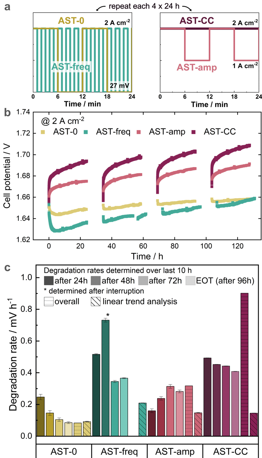
Fig. 1 (a) Four different ASTs used in this study. Each was repeated four times for 24 h with intermittent characterization throughout the different stress tests. (b) Potential evolution throughout the different stress tests. (c) Degradation rates calculated with the potential at beginning (BOT) and end of test (EOT) (called 'overall'), from linear trend analysis and within each 24-h step. Within each 24-h period, the last 10 h were used for a linear fit, and the slope \pm standard deviation is shown. Each experiment was performed with pristine CCMs with Ir black-based anode ( 1.65 \pm 0.09 \text{ mg}_{\text{Ir}} \text{ cm}^{-2} ), Nafion NR212 membrane ( \sim 51 \mu\text{m} ) and Pt/C-based cathode ( 0.15 \pm 0.06 \text{ mg}_{\text{Pt}} \text{ cm}^{-2} ). The anode features a Pt-coated Ti-fiber transport layer (2GDL10-0.25) and the cathode a carbon-based transport layer (H24C5). All cells were operated at 80^\circ\text{C} with 100 \text{ ml min}^{-1} water supply to the anode and a dry cathode.
