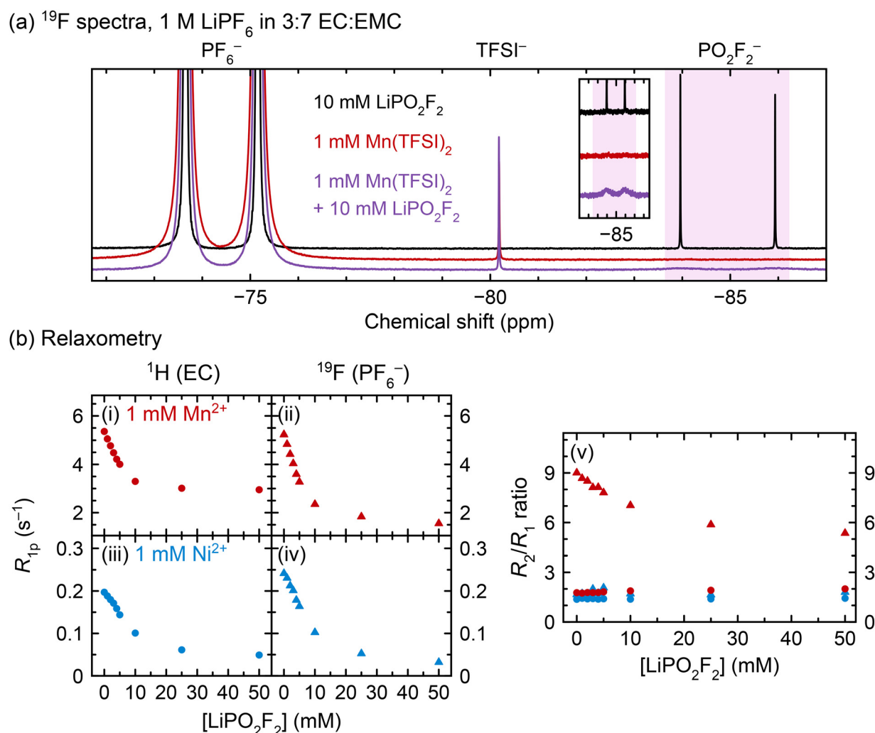
Fig. 5 (a) ^{19}\text{F} spectra and (b) ^1\text{H} EC and ^{19}\text{F} \text{PF}_6^- relaxation data of pristine electrolyte solutions to which \text{LiPO}_2\text{F}_2 was added. ^{19}\text{F} spectra are shown for solutions containing \text{LiPO}_2\text{F}_2 , \text{Mn}^{2+} , or both; inset shows enlargement of the \text{PO}_2\text{F}_2^- resonance. Longitudinal paramagnetic relaxation rates ( R_{1p} ) and R_2/R_1 ratios are shown for the ^1\text{H} EC (circles) and ^{19}\text{F} \text{PF}_6^- resonances (triangles), in solutions containing \text{Mn}^{2+} (red) or \text{Ni}^{2+} (blue). Electrolyte solutions comprised 1 M \text{LiPF}_6 in 3 : 7 EC : EMC (v/v).
