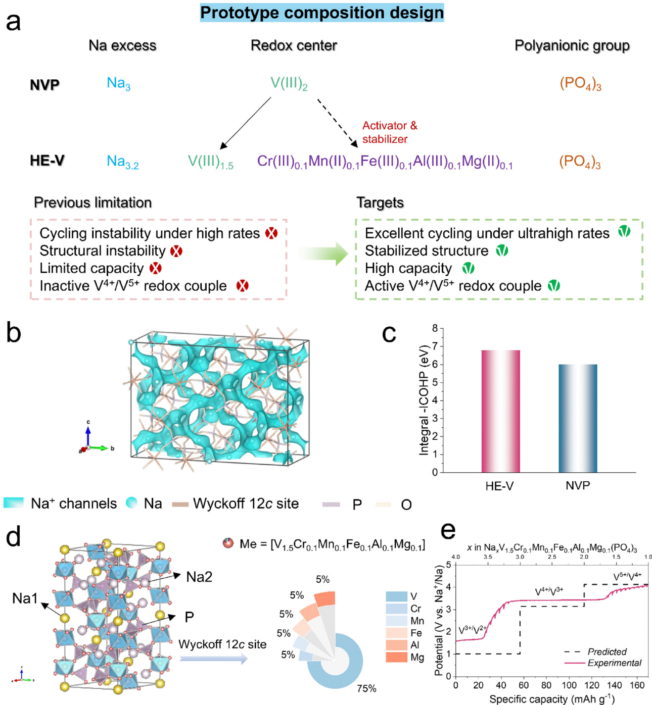
Fig. 1 Composition design principle and theoretical studies of physicochemical properties. (a) Prototype composition design principle. (b) Na + ion diffusion pathways (blue isosurface) in HE-V from the BV calculation. (c) Integral ICOHP values of all V–O bonds in HE-V and NVP. (d) Illustrations of crystalline structures and transition metal compositions in HE-V. (e) Calculated voltage profile.
