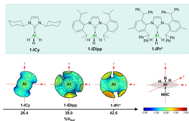
Fig. 2 Topographic steric maps of NHC ligands in 1-ICy , 1-IDipp and 1-IPr* . The iso-contour curves of the steric maps are in \text{\AA} .
