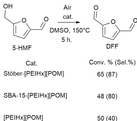
Scheme 3 Direct oxidation of 5-HMF catalysed by SiO 2 -[PEIH] x [PMO] y . Reaction conditions: 140 mg of 5-HMF (1.11 mmol), 22.5 mg of SBA-15-[PEIH] x [PMO 12 O 40 ] (0.06 mol% [PMO 12 O 40 ], 0.7 mol% Mo), 22.5 mg of Stöber-[PEIH] x [PMO 12 O 40 ] (0.05 mol%, PMO 12 O 40 , 0.6 mol% Mo) or 1.2 mg of [PEIH] x [PMO 12 O 40 ] (0.05 mol%, PMO 12 O 40 , 0.6 mol% Mo), 6 mL of solvent, 65 mg of naphthalene as the internal standard. Conversion and selectivity were determined by GC-FID.
