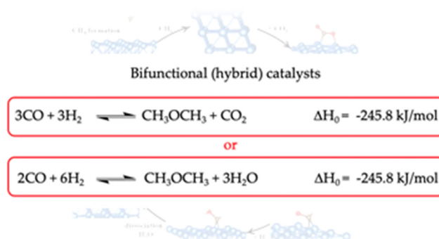
Fig. 2 Alternative (direct) one-step process DME synthesis.
