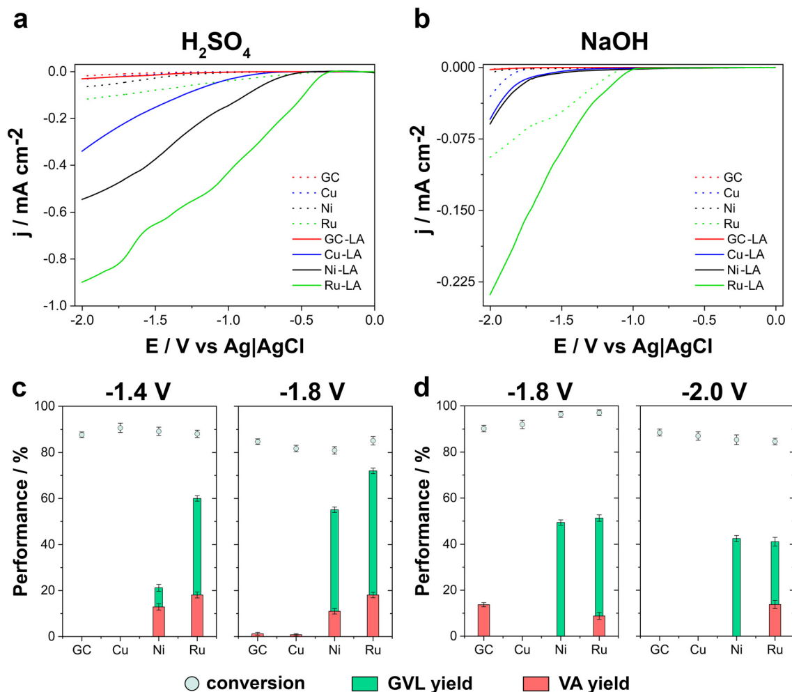
Fig. 2 Linear sweep voltammograms (LSV) recorded within a potential range of 0.0 V to -2.0 V vs. Ag|AgCl|Cl ^{-} at 50 mV s ^{-1} , in the absence (dashed line) and presence (solid line) of 0.5 M of LA, using Cu, Ni, Ru, and bare GC electrodes in (a) acidic and (b) alkaline media. Conversion percentages and product selectivity toward GVL and VA in (c) acidic and (d) basic media. All experiments were performed in triplicate, with values reported as the mean \pm standard deviation.
