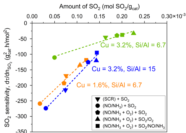
Fig. 5 \text{SO}_2 sensitivity as function of total \text{SO}_2 uptake after 6 cycles under different conditions (see also Fig. 3).
