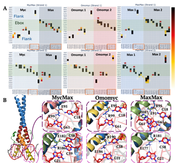
Fig. 5 Protein–DNA hydrogen bond (HB) interactions and patterns in the MycMax, Omomyc dimer, and MaxMax complexes. (A) Heatmaps of HB occupancy for MycMax, Omomyc, and MaxMax complexes interacting with the DNA from individual 1-μs MD simulations. HB contacts with the DNA bases are marked with red stars. The E-box region is highlighted in green, and each protein monomer is delimited by a rectangular colored box. The HLH region is delimited by an orange box on the x-axis. (B) Molecular visualization of key protein–DNA HBs. Each monomer is shown in a separate row. The top row shows Myc, Omo1 and Max1, respectively. The bottom row shows Max, Omo2, and Max2, respectively.
