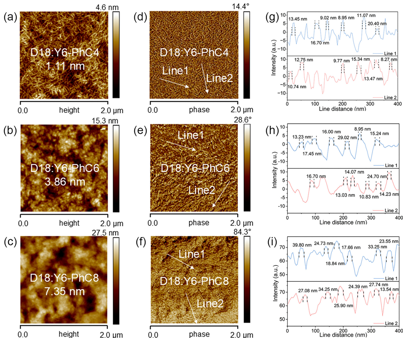
Fig. 3 AFM height images of (a) D18:Y6-PhC4, (b) D18:Y6-PhC6 and (c) D18:Y6-PhC8 blend films. AFM phase images of (d) D18:Y6-PhC4, (e) D18:Y6-PhC6 and (f) D18:Y6-PhC8 blend films. Line profiles along the location of the solid white lines in the panels to obtain the grain sizes in (g) D18:Y6-PhC4, (h) D18:Y6-PhC6 and (i) D18:Y6-PhC8 blend films. The nano-grain size in each case was specifically calculated from the FWHM (the distance between two adjacent dashed lines in the graphs).
