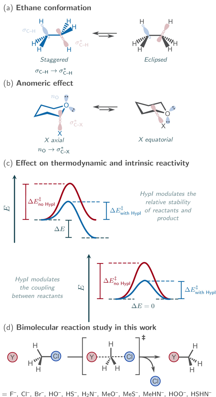
Figure 1: (a) and (b) Representative configurational processes stabilized by hyperconjugative interactions (Hypl); the most stable conformers are highlighted in blue. (c) Conceptual illustration of how hyperconjugation can modulate both thermodynamic parameters (e.g., reaction energies) and intrinsic barriers. (d) Schematic representation of the \text{S}_{\text{N}}2 reaction under investigation, including the series of nucleophiles considered in this study.
