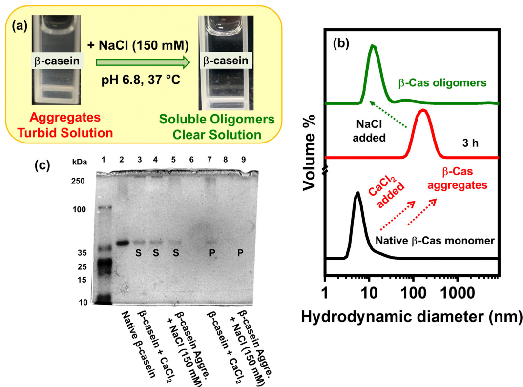
Fig. 1 Disruption of \text{Ca}^{2+} -induced \beta -casein aggregates formed at pH 6.8, 37 °C upon the addition of 150 mM sodium chloride (NaCl) to the preformed aggregates. (a) Disappearance of the solution turbidity, observed visually, resulting in a clear solution. (b) Hydrodynamic diameter of the native \beta -casein (black) and \beta -casein aggregates (red) formed after 3 h of incubation in the presence of 2.5 mM \text{CaCl}_2 , pH 6.8, 37 °C, monitored using dynamic light scattering (DLS), depicted by a stack-plot representation. A significant reduction in the hydrodynamic diameter of \beta -casein aggregates, upon the addition of 150 mM NaCl (shown by a green dashed arrow), indicates dissolution of the aggregates leading to aggregation-incompetent, soluble oligomers (green). (c) Native-PAGE analyses of native \beta -casein monomer (lane 2), \text{Ca}^{2+} -induced \beta -casein aggregates formed at ~37 °C (lanes 3 and 7) and upon the addition of 150 mM NaCl (post-addition approach) into the preformed \beta -casein aggregates after 3 h of incubation (lanes 5 and 9) (S: supernatant, P: pellet).
