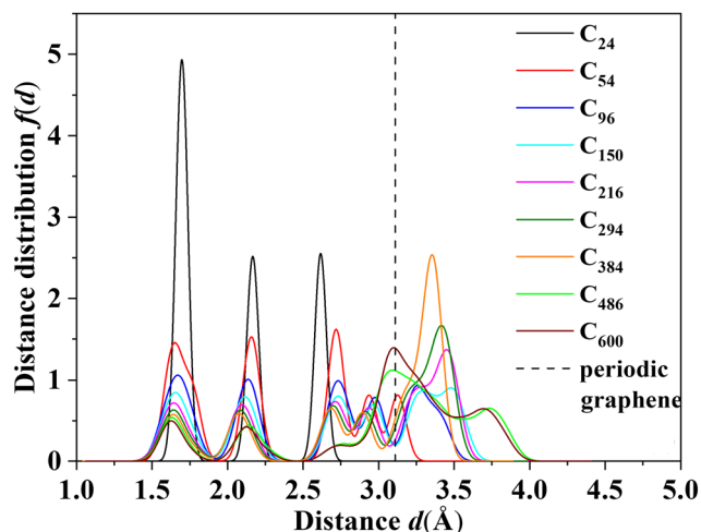
Fig. 6 Distance distribution of graphene nanosheets from the Cu(111) surface.
