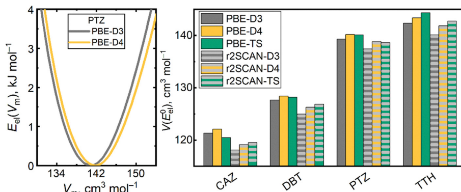
Fig. 3 Illustration of how static electronic energies E_{\text{el}} modelled by PBE-D3 and PBE-D4 for phenothiazine vary with respect to the molar volume V_m of the crystal (left); and a comparison of molar-volume coordinates V_0 of the minimum points of E_{\text{el}}(V_m) curves calculated for the target crystal forms using either PBE or r^2 SCAN functionals coupled with either D3, D4 or TS dispersion models (right).
