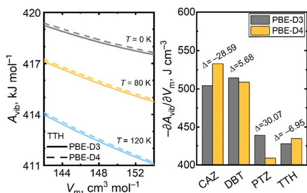
Fig. 4 Illustration of the vibrational Helmholtz energy of crystalline thianthrene as a function of molar volume at selected temperatures (left) and a comparison of the slopes of A_{\text{vib}}(V_m) functions calculated using either the PBE-D3 or PBE-D4 models for all the target materials at 298 K and at predicted equilibrium volumes corresponding to the standard pressure. Value \Delta represents the A_{\text{vib}}(V_m) slope from PBE-D3 minus that from PBE-D4, in \text{J cm}^{-3} (right).
