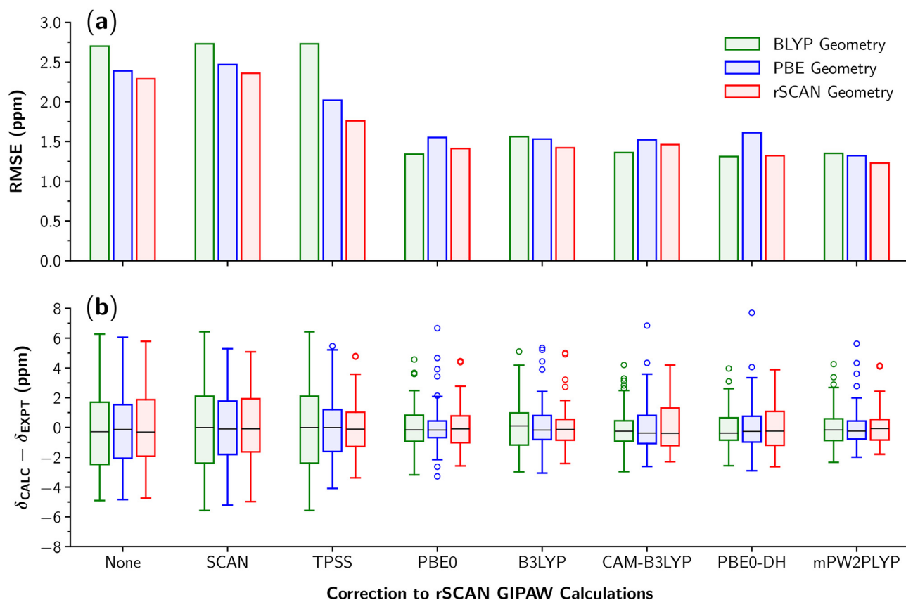
Correction to rSCAN GIPAW Calculations
