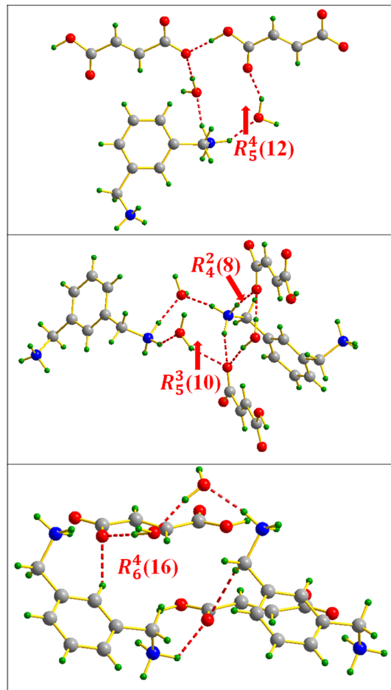
Fig. 21 Supramolecular synthons resulting from the FA...MXDA...water interaction in m -xylylenediamine/fumaric acid-trihydrate salt (IV).
