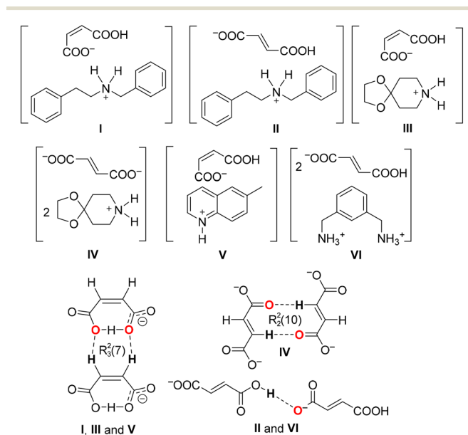
Scheme 1 Salts reported in this manuscript and motifs studied computationally.
