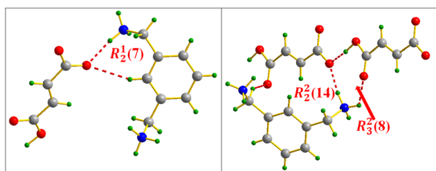
Fig. 20 FA...MXDA intermolecular interaction motifs in m -xylylenediamine/fumaric acid-trihydrate salt (IV).
