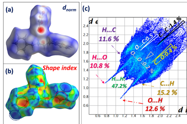
Fig. 3 Hirshfeld surface analysis shown in d_{\text{norm}} (a) and shape index (b) modes for compound I and computed fingerprint plots (c).
