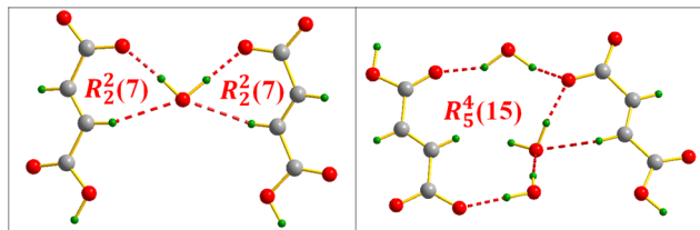
Fig. 19 Supramolecular synthons formed via the FA...water intermolecular interaction in m -xylylenediamine/fumaric acid-trihydrate salt (IV).
