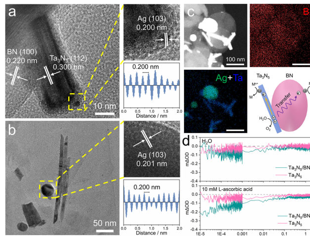
Fig. 3 HRTEM images and lattice fringe distances of the Ag particles loaded on (a) \text{Ta}_3\text{N}_5 and (b) BN in the \text{Ta}_3\text{N}_5/\text{BN} particles. (c) Dark field image, EDS mappings and structure diagram of the \text{Ta}_3\text{N}_5/\text{BN} sample loaded with Ag. (d) Transient absorption spectrum for \text{Ta}_3\text{N}_5 and \text{Ta}_3\text{N}_5/\text{BN} in water without (top panel) or with L-ascorbic acid (bottom panel). The pump and probe lights in (d) are 355 and 580 nm, respectively. The \text{Ta}_3\text{N}_5/\text{BN} sample is prepared from a Ta : BN = 2 : 10 ratio.
