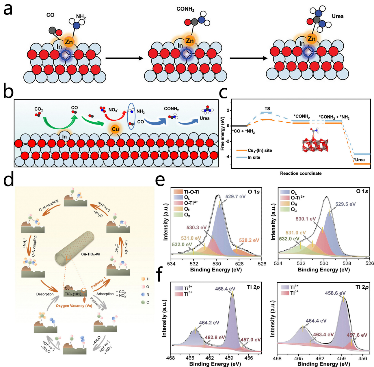
Fig. 10 (a) Schematic for the tandem UECN catalytic mechanism of \text{ZnI}/\text{In}_2\text{O}_{3-x} . Reproduced with permission from ref. 56. Copyright 2024, Advanced Energy Materials. (b) Schematic for the relay UENC catalytic mechanism of \text{CuI}/\text{In}_2\text{O}_3 . Reproduced with permission from ref. 57. Copyright 2024, ACS Nano. (c) Free energy diagrams for the electrocatalytic C–N coupling of ^*\text{CO} and ^*\text{NH}_2 on \text{In}_2\text{O}_3 and \text{CuI}/\text{In}_2\text{O}_3 . Reproduced with permission from ref. 57. Copyright 2024, ACS Nano. (d) Schematic diagram of \text{CuWO}_4 bimetallic alloys for highly efficient catalytic nitrate synthesis of urea. (e) O 1s XPS spectra comparing undoped \text{TiO}_2 and Cu-doped \text{TiO}_2 . (f) Ti 2p XPS spectra comparing undoped \text{TiO}_2 and Cu-doped \text{TiO}_2 . Reproduced with permission from ref. 58. Copyright 2020, Journal of Colloid and Interface Science.
