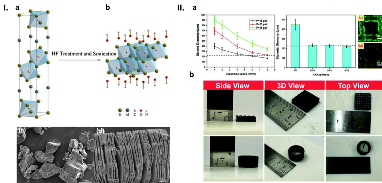
Fig. 32 (I) Preparation and structure of Ti_3C_2 MXene. (a) Crystal structure of Ti_3AlC_2 ; (b) chemical structure of Ti_3C_2 , with OH termination ( Ti_3C_2 was made from Ti_3AlC_2 by HF etching and sonication); (c) and (d) SEM images of exfoliated Ti_3AlC_2 by 49% HF at 60 °C for 24 h. In (c), a low magnification is presented to show all grains are exfoliated, and in (d) a high magnification is used to show a fully exfoliated grain. Reproduced from ref. 529 with permission from Elsevier; copyright © 2015 Elsevier B.V. (II) Evaluation of the printability of MXene nanocomposite ink. (a) Finding the optimised operating parameters for extrusion-based 3D printing. (b) Pictures of 3D-printed structures fabricated using the MXene nanocomposite ink containing 1 \text{ mg mL}^{-1} Ti_3C_2 MXene nanosheets. Reproduced from ref. 256 with permission from The Royal Chemical Society; copyright © 2020.
