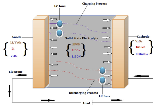
Fig. 2 Schematic of a representative lithium-based solid-state battery, showing the direction of ion movement and some of the possible anode, electrolyte, and cathode combinations (reproduced with permission from ref. 37).
