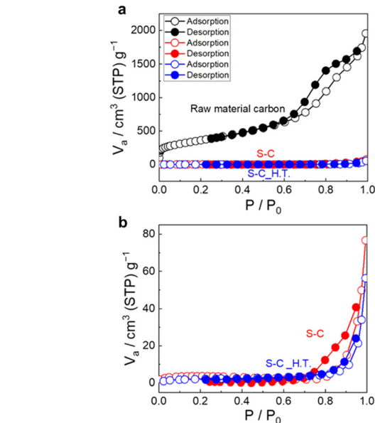
Fig. 3 (a) The \text{N}_2 adsorption/desorption isotherms of the raw material carbon, S-C and S-C_H.T. (b) The enlarged \text{N}_2 adsorption/desorption isotherms are also shown.
