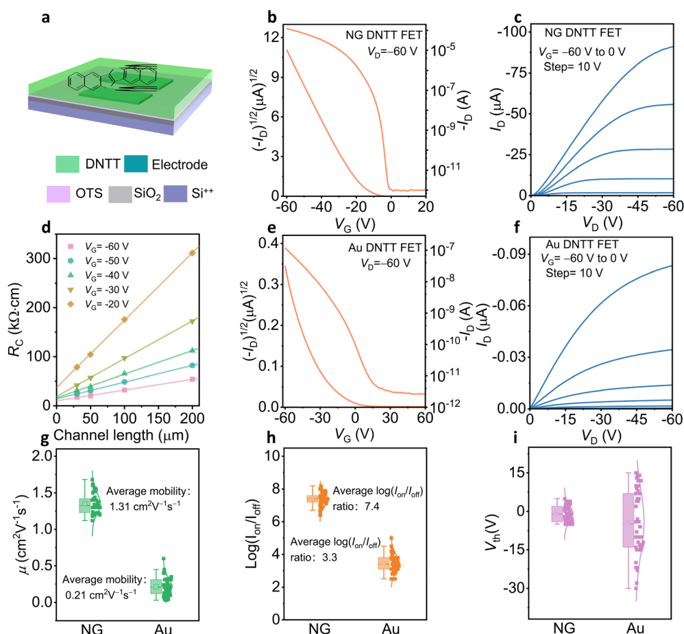
Fig. 3 Electrical performance of the NG and Au electrode DNNT OFETs. (a) Schematic diagram of the BGBC structure OFET, and chemical structure of DNNT. (b) and (e) Transfer characteristics of the NG and Au electrode DNNT OFETs measured in the saturated regime of operation ( V_D = -60 \text{ V} ), respectively. (c) and (f) Output characteristics of the NG and Au electrode DNNT OFETs, respectively. (d) R_C extraction using the TLM method from the NG electrode DNNT OFETs. (g)–(h) Statistics of mobility, on/off ratio ( I_{on}/I_{off} ), and threshold voltage ( V_{th} ) of 50 NG and Au electrode DNNT OFETs.
