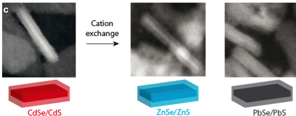
Fig. 11 (a) HAADF-STEM image of 2CdS/2ZnS/2CdS/4CdSe/2CdS/2ZnS/2CdS formed by c-ALD using Li 2 S/Li 2 Se and anhydrous Cd(HCOO) 2 /Zn(OAc) 2 powders as the sources of chalcogen and metal precursors, respectively; (b) the interplanar distances for this structure shown in (a); (c) schematic representation of the cation exchange of CdSe/CdS core/shell NPLs to ZnSe/ZnS and PbSe/PbS NPLs with corresponding HAADF-STEM images. Panels (a) and (b) are adapted with permission from The American Chemical Society. 240 Panel (c) is adapted with permission from The American Chemical Society. 254
