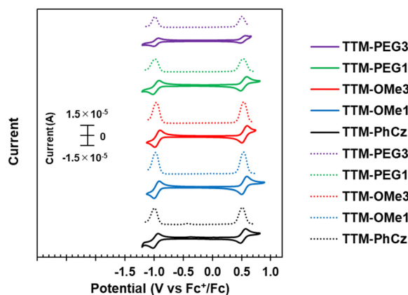
Fig. 6 (Solid line) Cyclic voltammogram (CV) and (dotted line) differential pulse voltammogram (DPV) of TTM-Cz derivatives in \text{CH}_2\text{Cl}_2 .
