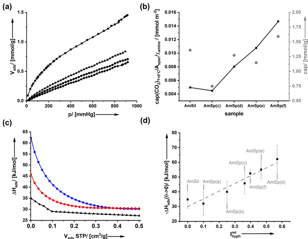
Fig. 4 (a) CO 2 adsorption isotherms of AmSp(d)Sil measured at T = 0\text{ }^{\circ}\text{C} (squares), 30\text{ }^{\circ}\text{C} (triangles), 40\text{ }^{\circ}\text{C} (circles) and 50\text{ }^{\circ}\text{C} (hashes). (b) Comparison of the CO 2 uptake capacity between different organosilica materials; grey circles = capacity in mmol CO 2 per gram material; black line = data referenced to A_{\text{spec}} and \chi_{\text{amine}} of the respective sample. (c) isothermic heat of CO 2 adsorption determined from T -dependent adsorption measurements for three exemplary materials; black triangles = AmSil; red circles AmSp(c); blue squares AmSp(d). (d) Correlation between the isothermic adsorption heat of CO 2 on different organosilica aerogels and the correlation with the relative hydrophobicity index I_{\text{hyp}}^{\text{rel}} .
