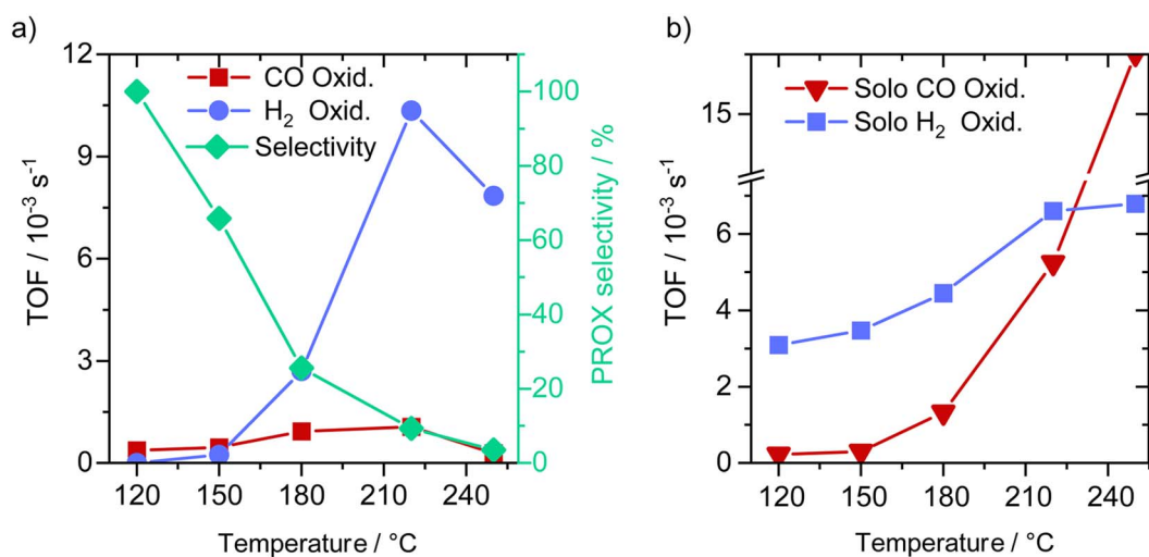
Fig. 2 (a) CO and H 2 oxidation reactions during the PROX reaction (1% CO, 1% O 2 , 80% H 2 and N 2 ) at different temperatures, after the H 2 50 pretreatment (1 h in 10% H 2 /N 2 at 250 °C) and (left y-axis) corresponding selectivity for CO oxidation derived from rates of CO 2 and H 2 O formation (right y-axis). (b) Solo CO oxidation (1% CO, 1% O 2 , and N 2 ) and hydrogen oxidation (1% O 2 , 80% H 2 and N 2 ) reactions after H 2 50 treatments.
