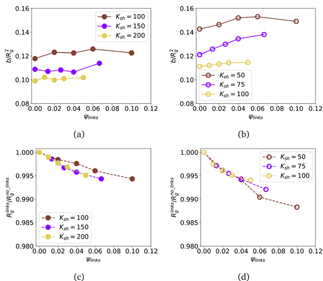
Fig. 3 Rescaled asphericity b/R_g^2 ((a) and (b)), and relative change of the gyration radius R_g^{\text{links}}/R_g^{\text{no-links}} of core-shell nanogels in a good solvent with different fractions of cross-linked monomers \psi_{\text{links}} . The shell consists of K_{\text{sh}} polymer chains, as indicated in the legend. R_g^{\text{no-links}} is the gyration radius of a core-shell nanogel with a non-cross-linked shell. (a) and (c) M_{\text{sh}} = 10 ; (b) and (d) M_{\text{sh}} = 20 . Brown corresponds to nanogels with N^{\text{sh}} = 1000 ; purple – N^{\text{sh}} = 1500 ; yellow – N^{\text{sh}} = 2000 .
