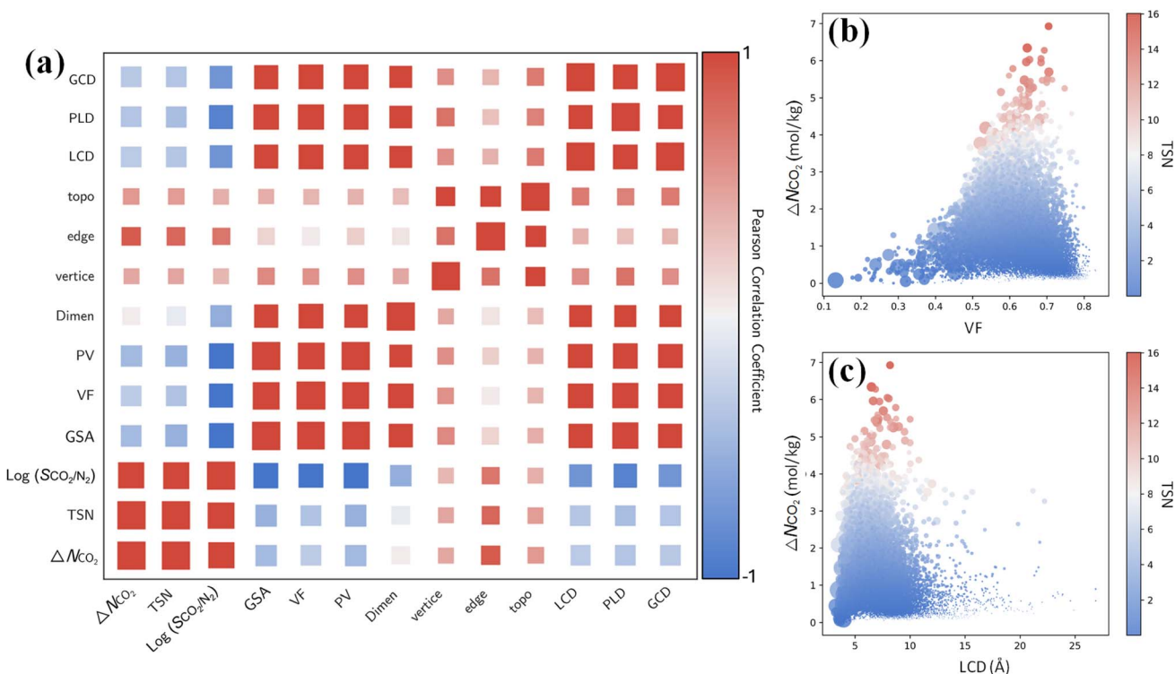
Fig. 7 (a) Pearson correlation matrix (PCM) between CO 2 capture performance metrics ( \Delta N_{CO_2} , TSN and \log(S_{CO_2/N_2}) ) and structural characteristics (GSA, VF, PV, dimensionality, vertex, edge, topology, LCD, PLD and GCD). (b and c) Relationships of \Delta N_{CO_2} with the VF and LCD in 17 173 MOFs, with color-coding based on TSN.
