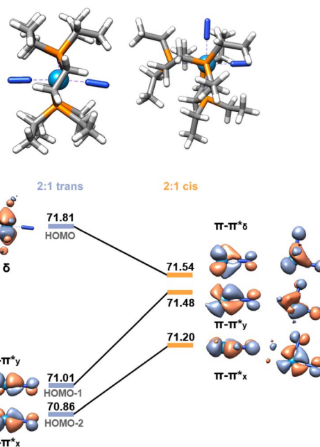
Fig. 7 Cis (11Al) vs. trans (8Al) frontier orbitals (HOMO to HOMO–2). AICF omitted for clarity. Orbitals of the cis isomer are shown in side and top views.
