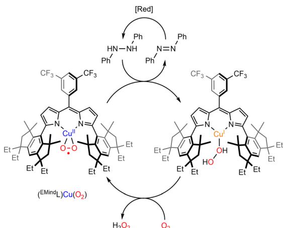
Scheme 7 Reaction of [(^{E\text{Mind}}\text{L})\text{Cu}^{\text{II}}(\text{O}_2)] with 1,2-diphenylhydrazine to produce azoarene and [(^{E\text{Mind}}\text{L})\text{Cu}^{\text{II}}(\text{H}_2\text{O}_2)] . Adapted from ref. 83.
