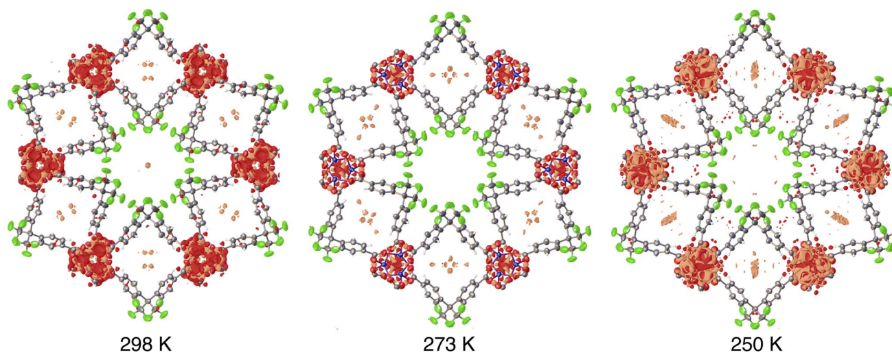
Fig. 4 Residual electron density within \text{CF}_4 -dosed Zn(fba). A crystal of Zn(fba) housed within a borosilicate capillary was dosed with 1 bar \text{CF}_4 at ambient temperature, flame sealed, and mounted onto a diffractometer goniometer head. Data collection was performed at 298 K, 273 K, and 250 K. The capillary was allowed to equilibrate for at least 2 h at the analysis temperature prior to data collection. Orange and red regions correspond to positive and negative residual density, respectively. Electron density maps were generated using the Olex2 software package. 51 Isosurface values are set at 0.28 \text{ e } \text{\AA}^{-3} .
